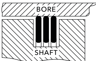
Single-Turn, Three Ring Sets YH Series / QH Series
