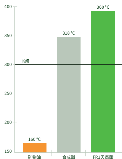
绝缘液燃点对比
