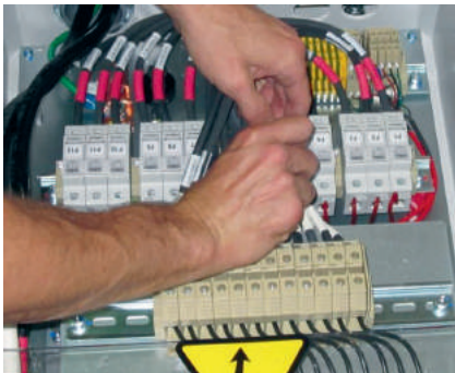
Electrical Cabinet
